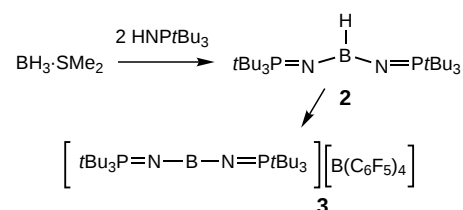
Scheme 2. Synthesis of 2 and its conversion to 3 .
